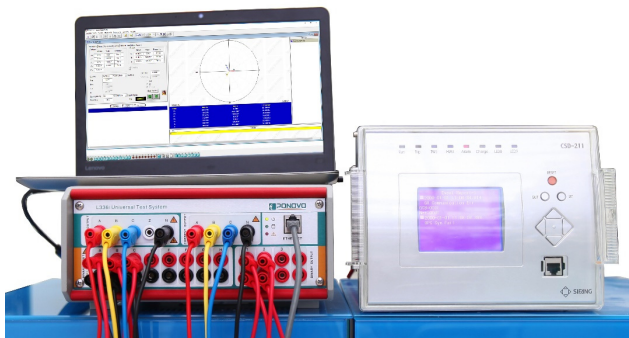
L336i-E with PC Powertest software for testing relay
